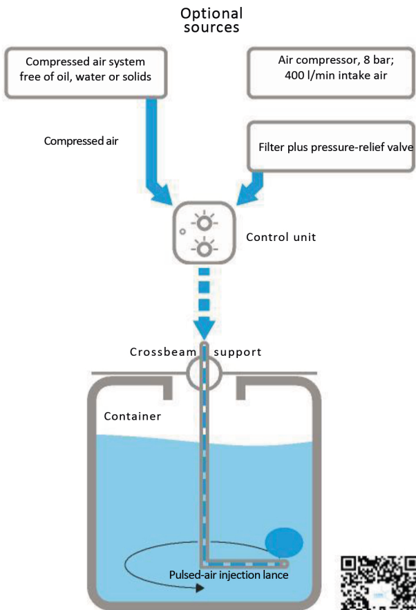
Crossbeam support
